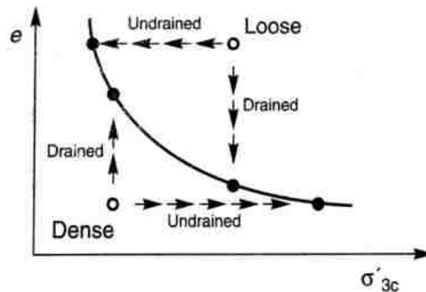
Figure 3-2: Behavior of initially loose and dense specimens under drained and undrained conditions (Kramer, 1996).
